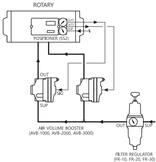
ROTARY ACTUATOR
