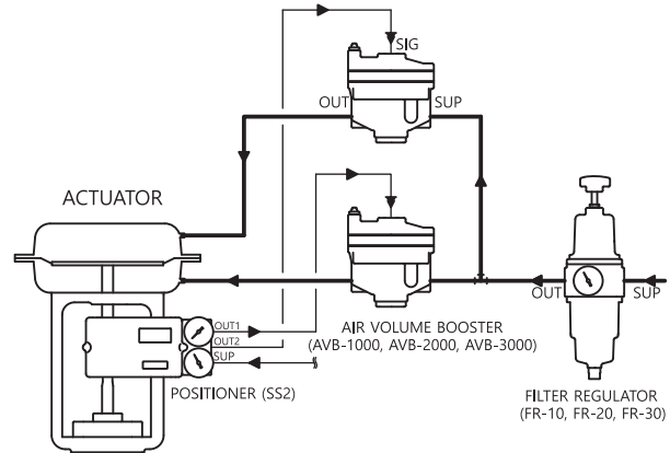
DOUBLE ACTING
